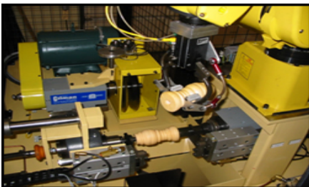
Robotic Load/Unload
